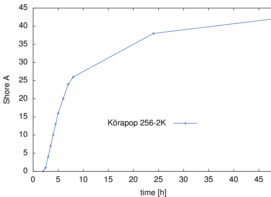
Figure 1: curing of Körapop 256-2K, build up of Shore A at 23°C
